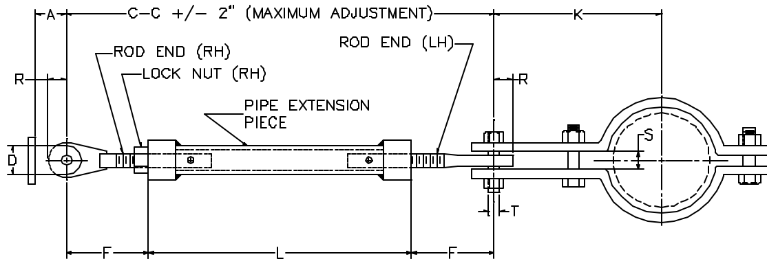
FIG. 320 THREADED SWAY STRUT ASSEMBLY WITH FIELD WELDED EXTENSION PIECE (ALTERNATE DESIGN)
