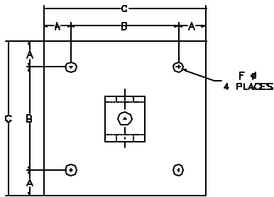
FIG. 524 CONCRETE ATTACHMENT PLATE W/ BEAM BRACKET
