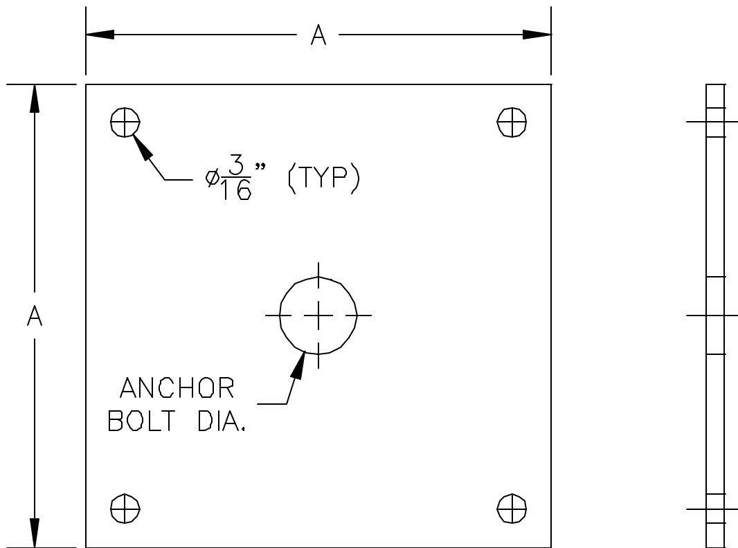
FIG. 900 CONCRETE INSERT PLATE FOR ANCHOR BOLT
