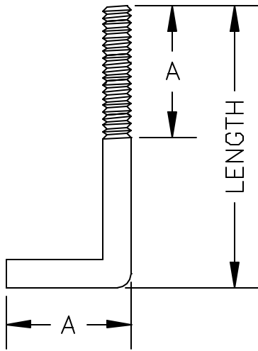
FIG. 945 ANCHOR BOLT – L – THREADED ONE END
